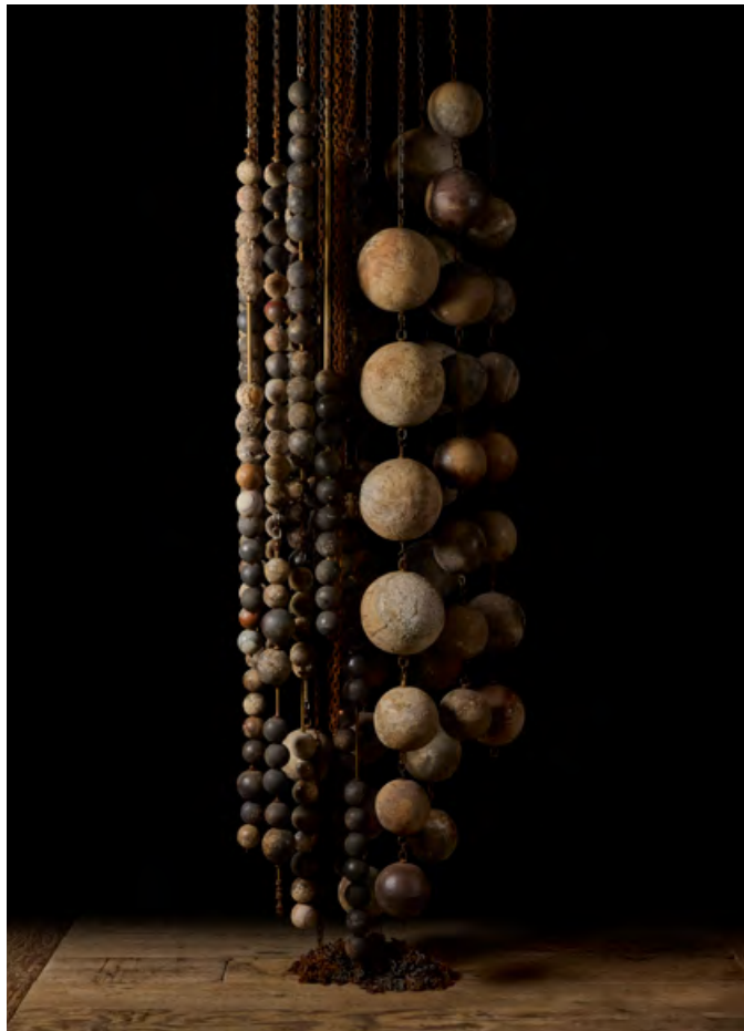
GRAVITY
